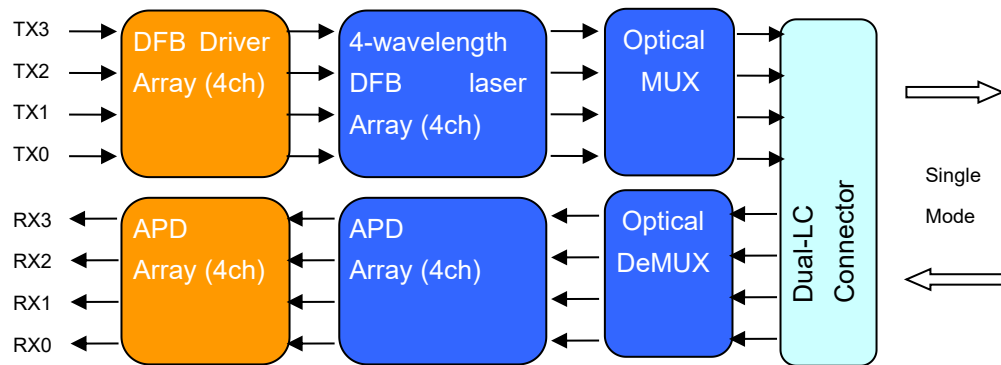
Figure 1: 40Gb/s QSFP ZR4 Lite Transceiver Block Diagram
